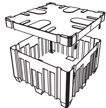
Exterior dimensions: Model UF4848: 51.5" x 51.5" x 30.5"-33.5" high
